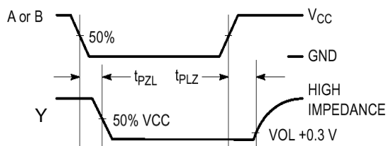
Figure 4. Switching Waveforms
